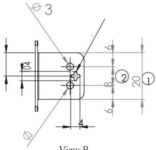
View B (Fixed to Scanner side)
