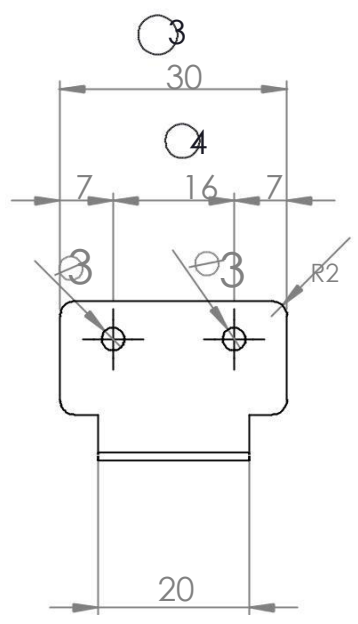
View A (Fixed to Host side)
